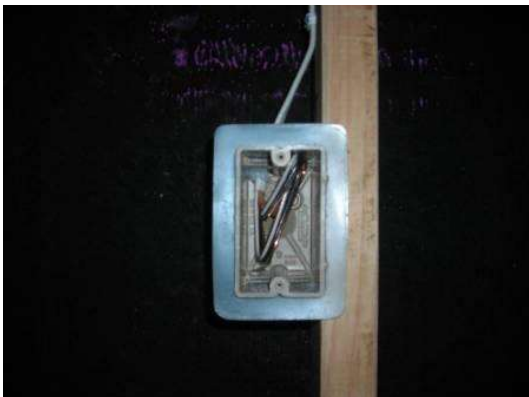
3. Gasketed boxes required in exterior walls where insulated with fiberglass.
