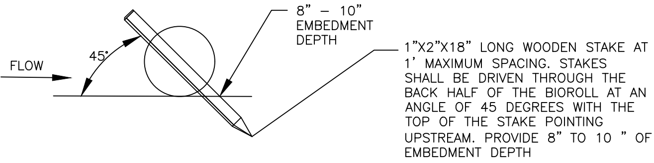
BIOROLL STAKE DETAIL
