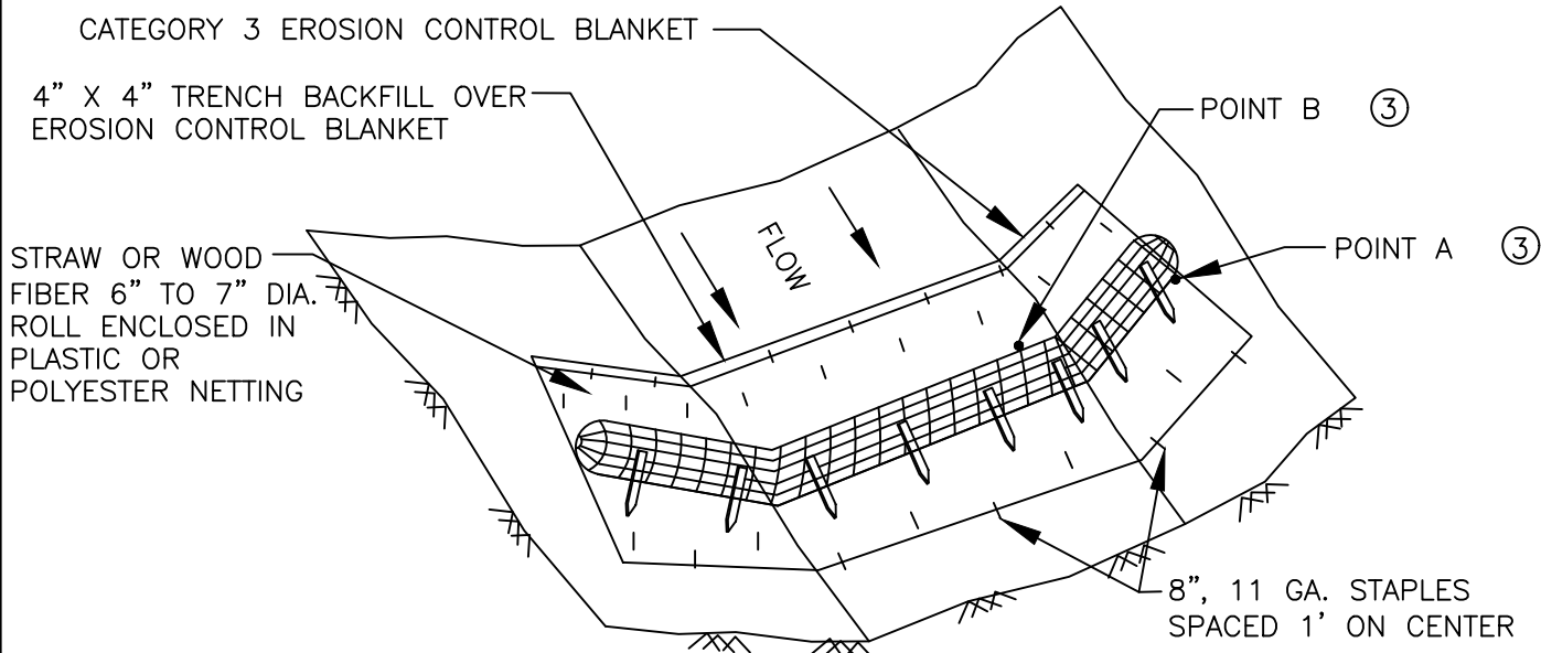
BIOROLL BLANKET SYSTEM DITCH CHECK (USE ON ROUGH GRADED AREAS)
